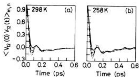
Figure 2. Time dependence of the correlation function of relative velocity of two water molecules which were hydrogen-bonded at time t = 0 . The solid, short-dashed, dotted and long-dashed curves correspond to the hydrogen-bonding states of the water pair (m, n) = (2, 2), (3, 3), (4, 4) and (5, 5) respectively.
